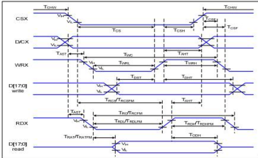
Figure 1 Parallel Interface Timing Characteristics (8080-Series MCU Interface)
