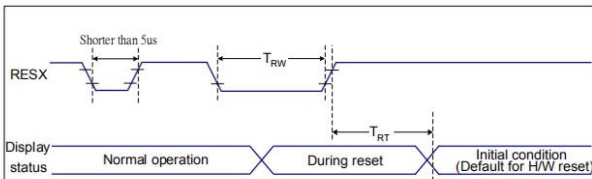
Reset Timing
